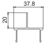
DGC4419 50 AW Stop
