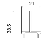
CSG715 50mm AW Stop
