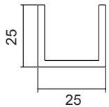
CH3218 Glazing Channel 25 x 25 x 3mm
