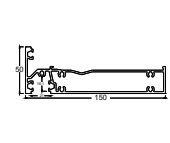
FGS632 Trans. Sill Internal Bead
