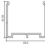
TJ731 Electric Winder Base
