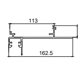
TJ686 SPANDRAL Subsill*
