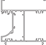
VEN005 Ventient 100mm Adapt.
