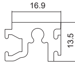
DGF4510 16mm Glazing Pocket Reducer
