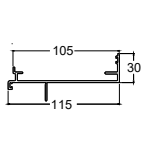
TJ370 Sub Sill with Reveal
