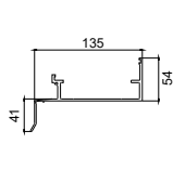
TJ479 High Perf. Sub Sill 22mm S.Back
