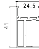
DT3207 Corner Receiver
