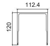
TJ520 120mm Sub Head
