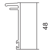
TJ6159 2 Part Sub Head/ Jamb Cover
