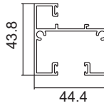
TJ226 45mm Mid Rail
