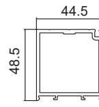
TJ220 Multi-Fold Door Stile
