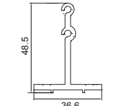
TJ212 Mid Rail Bracket
