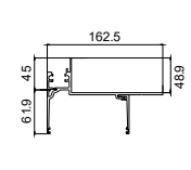
TJ687 SPANDRAL Sub- head*
