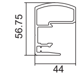
SW014 Medium Interlock
