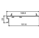
RWM053 Concealed Face Fix Adapter
