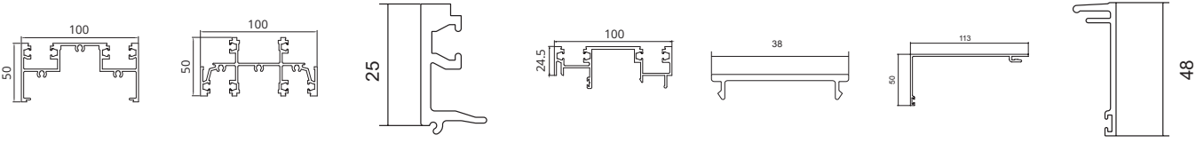
FGA100 Head/Jamb FGA102 Sill/Trans. FGS403 External Bead FGA104 Self Mating Mullion DGF4506 Pocket Filler TJ431 STD 2-Part Subhead / Jamb TJ6159 2 Part Sub Head / Jamb Cover
