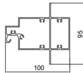
CSG729 100mm Hook AW Trans.
