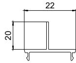
CDG4319 100mm CDG Clip-In AW Sash Stop
