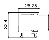
SWD623 Corner Meeting Stile
