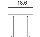
TJ307 Flush Pocket Filler
