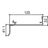
TJ379 H/D Sub Sill 12mm S.Back
