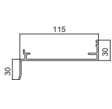
TJ368 Standard Sub Sill 6mm S.Back
