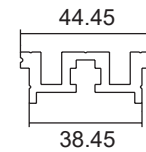
TJ361 Stacking Door Track
