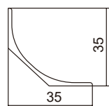
MC100 35mm Corner Mould
