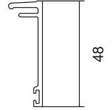
TJ6159 2 Part Sub Head / Jamb Cover
