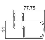
SWD032 Patio Door M/D Female Adapt.
