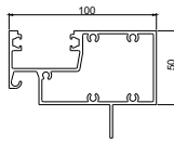
DGF4573 100mm Hook AW Head/Trans.
