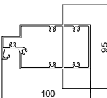
CSG729 100mm Hook AW Trans.
