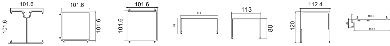
TJ308 Corner Post TJ319 Corner Post 90 Degree TJ347 180 Degree Post TJ309 49mm Sub Head TJ692 80mm Sub Head TJ520 120mm Sub Head RWM053 Concealed Face Fix Adapter
