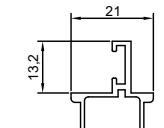
CSG306 40mm/45mm Door Stop
