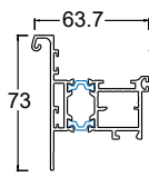
CG704 Hook AW Sash
