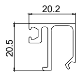
TJ716 16-22mm 50mm AW Bead
