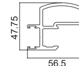
SW013 M/D Female Adapt.
