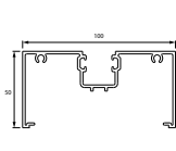
CSG301 100mm Standard M/ Frame
