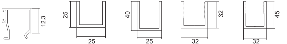
TJ202 Door Bead CH3218 Glazing Channel 25 x 25 x 3mm CH3220 Glazing Channel 25 x 40 x 3mm CH3232 Glazing Channel 32 x 32 x 3mm CH3245 Glazing Channel 32 x 45 x 3mm
