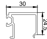
CGDG110 100mm Centre Bead
