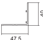
LVB040 40mm Weather Bar
