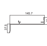
TJ432 Sub Sill 35mm S.Back
