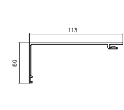
TJ431 Standard 2-Part Subhead/Jamb
