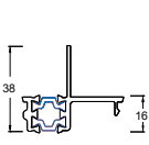
DTB026 AW Stop
