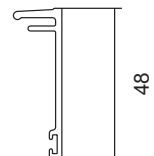
TJ6159 2 Part Sub Head / Jamb Cover
