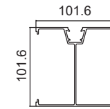
TJ308 Corner Post
