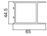
TJ207 Small Rail
