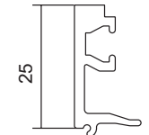
FGS403 External Bead
