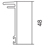
TJ6159 2 Part Sub Head/Jamb Cover
