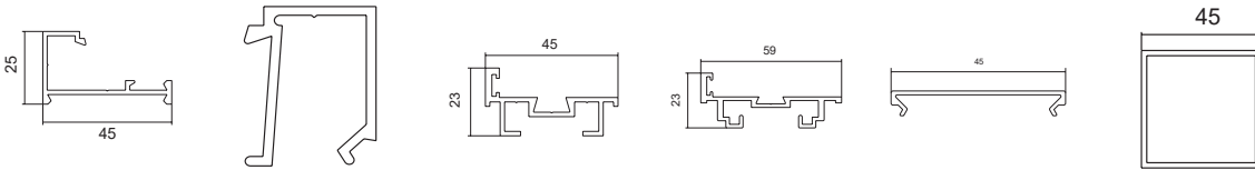
PS402 Standard 45mm Pocket Glazing PS403 Clip In Glazing Bead PS435 35mm Door Frame PS445 45mm Door Frame PS404 45mm End Cap SQ4545T16 Square Post
