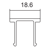
TJ307 Flush Pocket Filler
