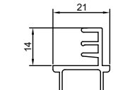
CSG031 45mm Door Stop
