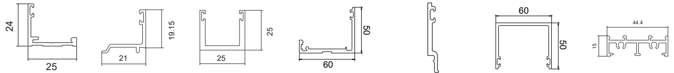
TJ015 Glazing Base 25 x 25 (Part 1) TJ016 Glazing Bead 25 x 25 (Part 2) TJ025 Glazing Channel 25 x 25 x 3mm TJ041 DG Channel Base - 50mm Pocket TJ042 DG Channel Bead - 50mm Pocket TJ043 DG Channel - 50mm Pocket TJ208 45mm Double Beaded Glazed Base
