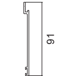
TJ324 Top Hung Door Track Cover
