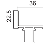
TJ720 35mm AW Stop
