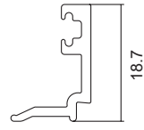
HV276 DG Multi-Fold Bead
