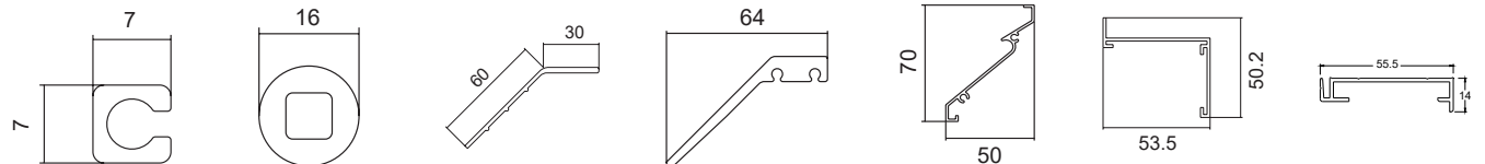
LV106 Louvre Fixing Rod LV107 Louvre Spacer Rod LV108 60mm Louvre Blade LV109 60mm x 10mm Blade LV050 50mm Louvre Blade LV051 50mm Louvre Frame LV052 Hinged D. Insert
