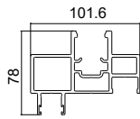
SWD039 Patio Door FSF Adapt.
