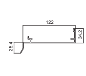
TJ359 L/D Sub Sill 12mm S.Back
