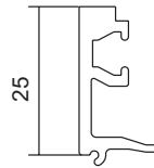
FGS403 External Bead
