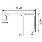
TJ714 6-12mm 50mm AW Bead
