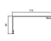
TJ431 Standard 2-Part Subhead / Jamb
