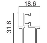
TJ306 45mm Door Stop
