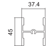
SD148 DG Architectural Door Midrail
