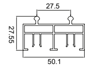
SWD619 Patio Door Fly Door Raised Clip-on Twin Track
