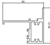
JS001 Jockey Sash
