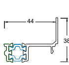
CG703 AW Clip-in Stop Front Glazed
