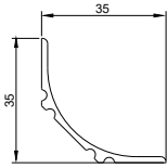
HIS118 Corner Mould
