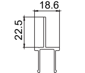
TJ715 50mm Clip-In AW Sash Stop
