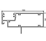
DGF6572 150mm Hook AW Head/Trans./Sill
