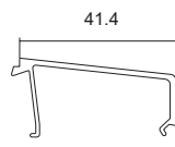
TJ303B Sill Bead - Sloping
