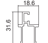
TJ306 45mm Door Stop
