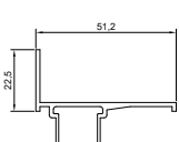
CSG720 35mm AW Stop
