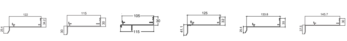
TJ359 L/D Sub Sill 12mm TJ368 Standard Sub Sill 0mm TJ370 Sub Sill with Reveal TJ379 H/D Sub Sill 12mm TJ259 Sub Sill 23mm S.Back TJ432 Sub Sill 35mm S.Back
