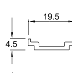
CGM001 Stay Packer
