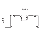
TJ301 101.6mm Standard M/Frame
