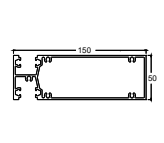
FGS631 AW Trans.
