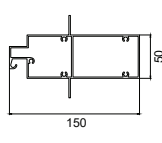
CDG6729 150mm Hook AW Trans.
