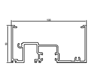
CSG346 Water-rated Head (In & Outward)
