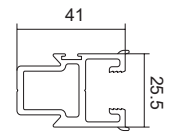
SW009 SG Interlock Stile
