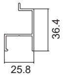
TJ737 Flyscreen Adapt./ Winder Support
