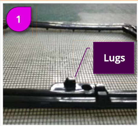
Turn screen spline side up; lug goes on spline side.
