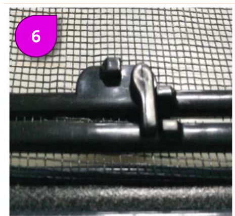
Finished lever position, spline side facing up.
