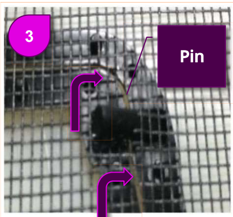
Cut mesh between and put pins under half of screen.
