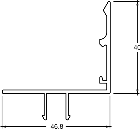
LCV005 HEAD WEATHER BAR
