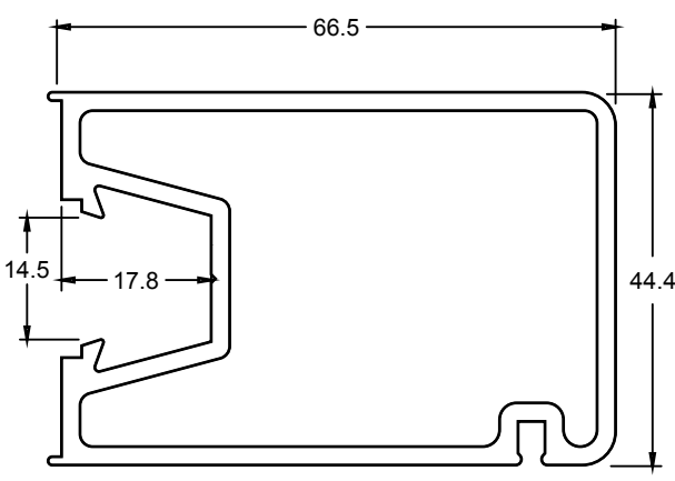
TJ322 SLIDING STILE
