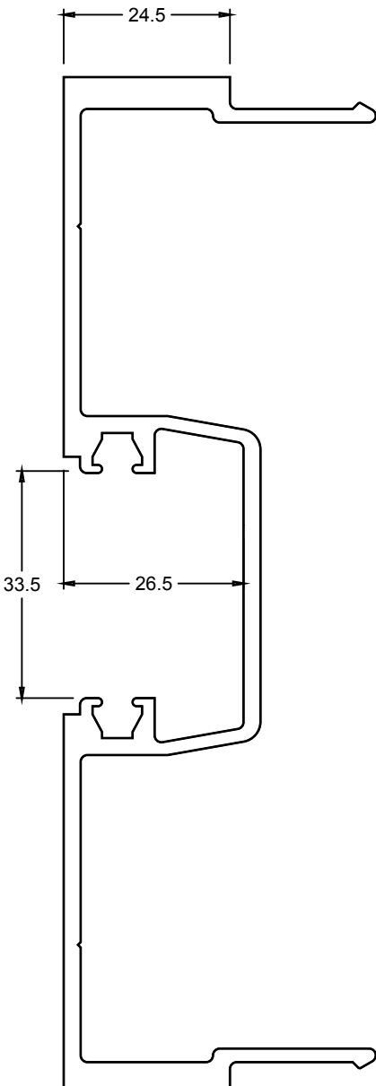
CDG6512 H/D SPLIT MULLION MALE
