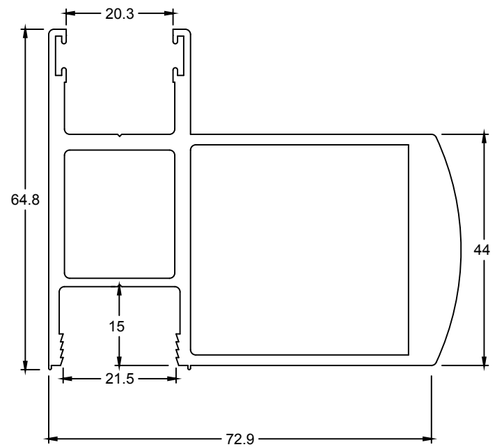
SWD065 DOUBLE GLAZED H/D FEMALE ADAPTER
