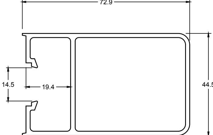
TJ443 PLAIN STILE
