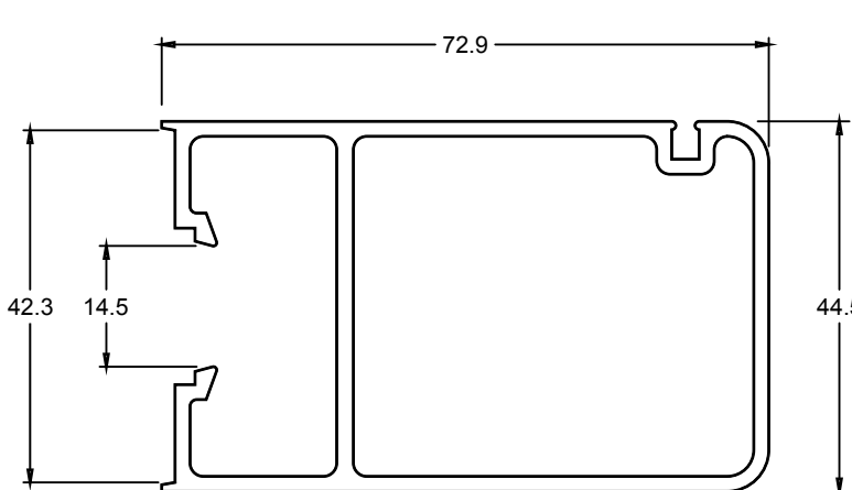
TJ442 SLIDING STILE
