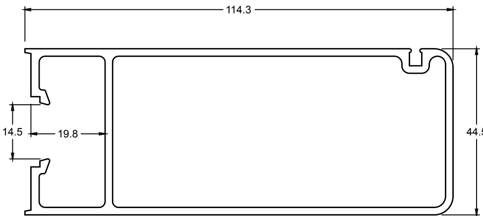
TJ452 SLIDING STILE
