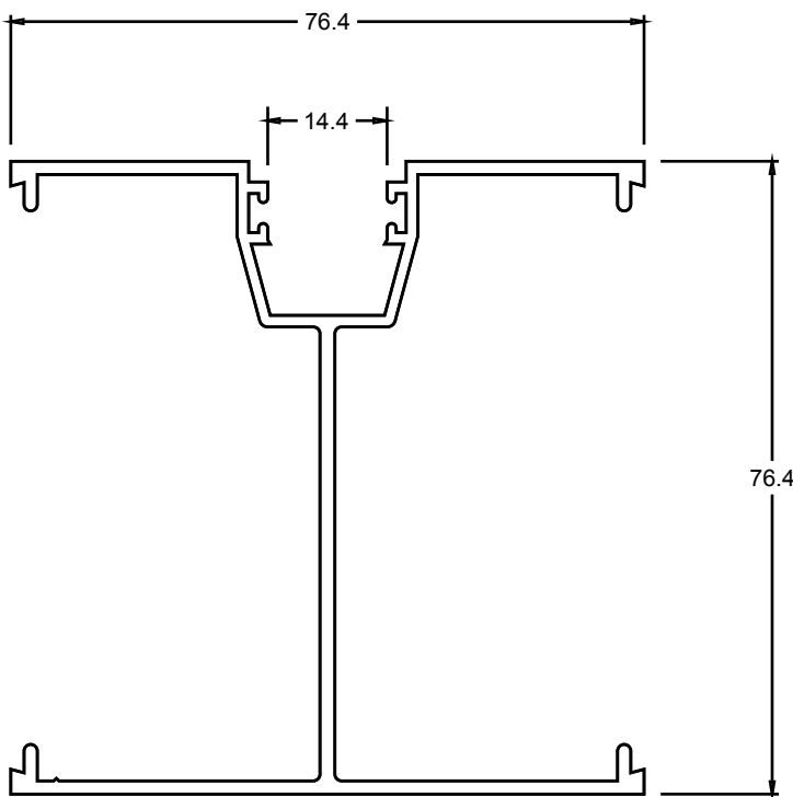
TJ718 CORNER POST
