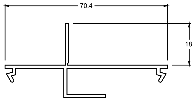
TJ751 REVEAL CLIP IN
