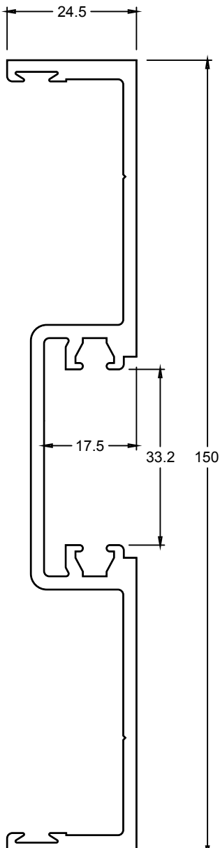
CDG6513 H/D SPLIT MULLION FEMALE
