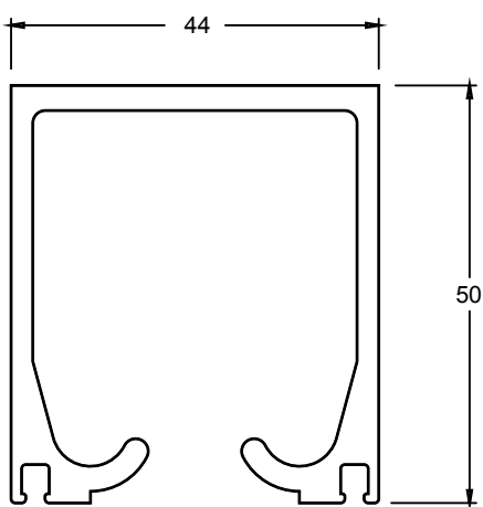
TJ343 TOP HUNG STACKING DOOR TRACK
