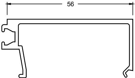
CDG6503 SILL BEAD
