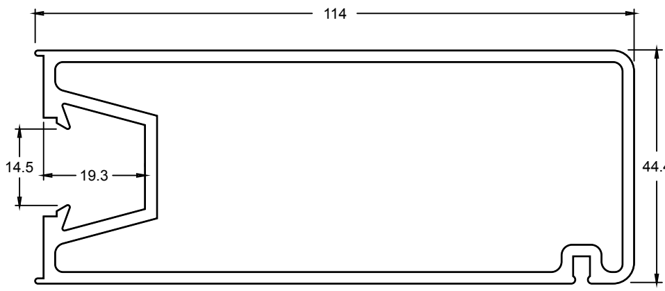
TJ159 SLIDING STILE
