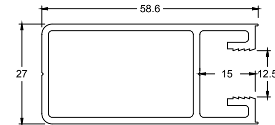
SWD056 S/G STILE
