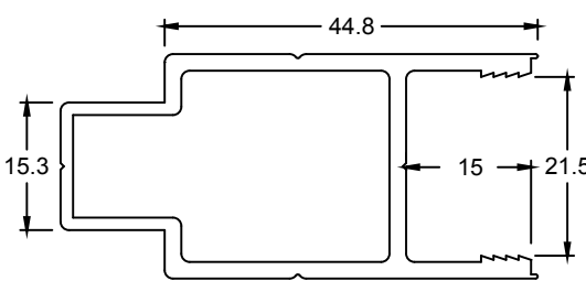
SWD067 MALE STILE
