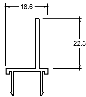
TJ730 35 AWNING STOP
