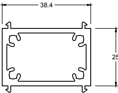
LVJ002 BOX GALLERY JOINER
