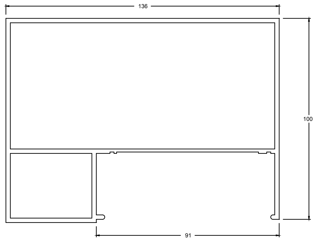
VEN001 VENT BOX (PRE-SLOTTED IN LEFT & RIGHT CONFIGURATIONS)
