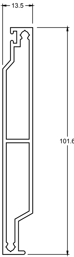
LVB1013 102 X 13.5mm BLADE
