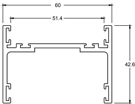
TJ328 DOOR GUIDE / RECEIVER
