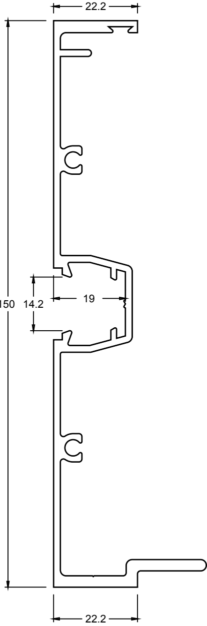
TJ6150 SELF MATING MULLION
