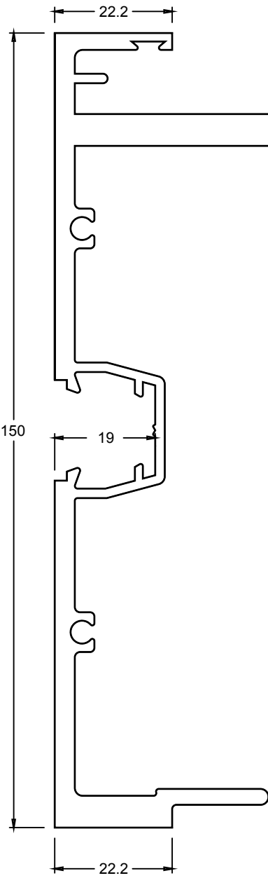
TJ6154 HD SELF MATING MULLION
