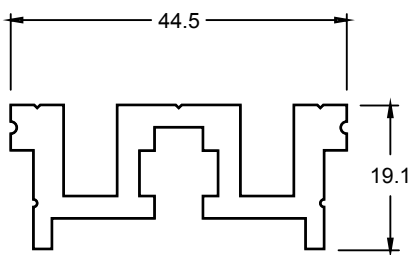
TJ361 STACKING DOOR TRACK
