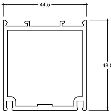
TJ211 MULTIFOLD DOOR STILE
