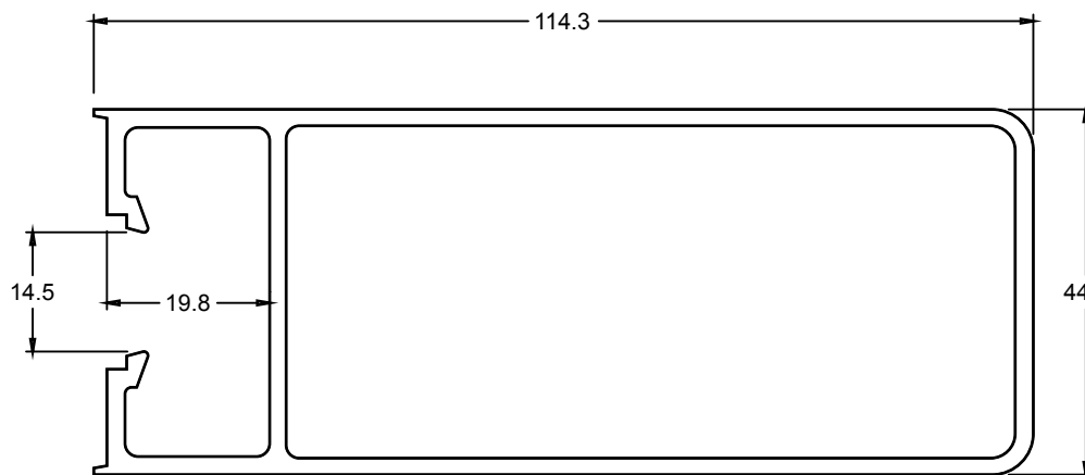
TJ453 PLAIN STILE
