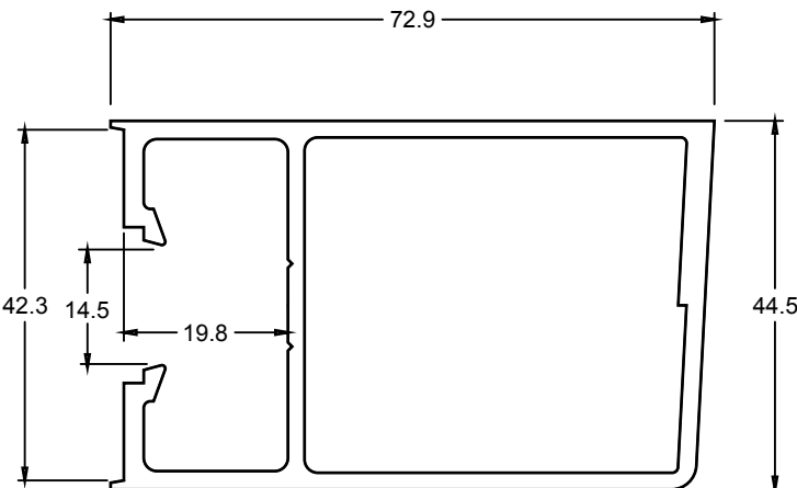
TJ441 HINGE STILE
