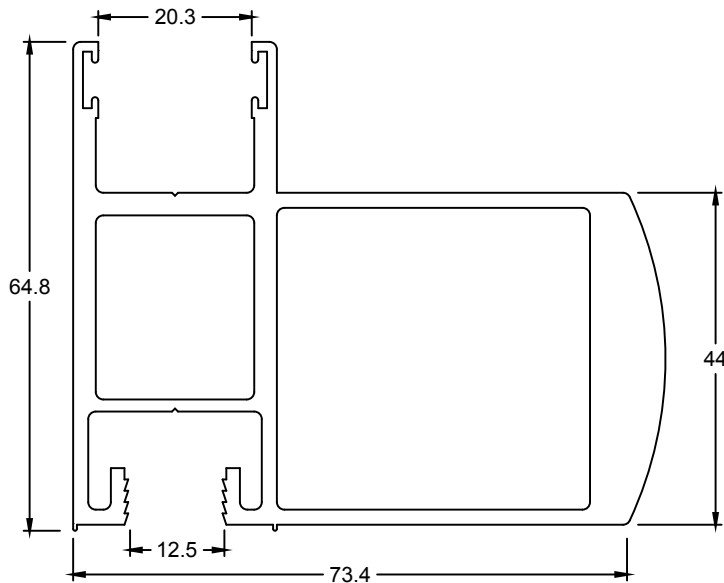
SWD055 SINGLE GLAZED H/D FEMALE ADAPTER
