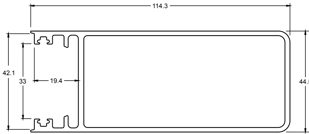
TJ437 PLAIN STILE
