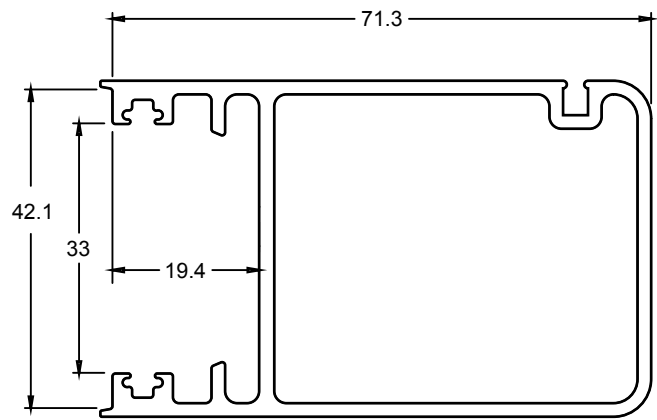
TJ416 LOCK STILE
