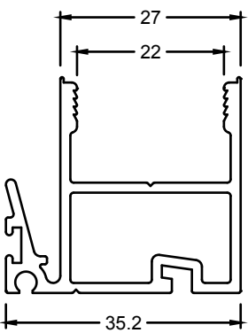
DH252 INTERLOCK BOTTOM SASH DG
