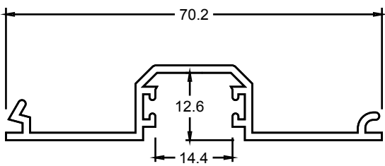
TJ704 GLAZING ADAPTOR
