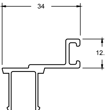
TJ6166 45mm DOOR STOP
