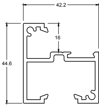
TJ326 MID RAIL
