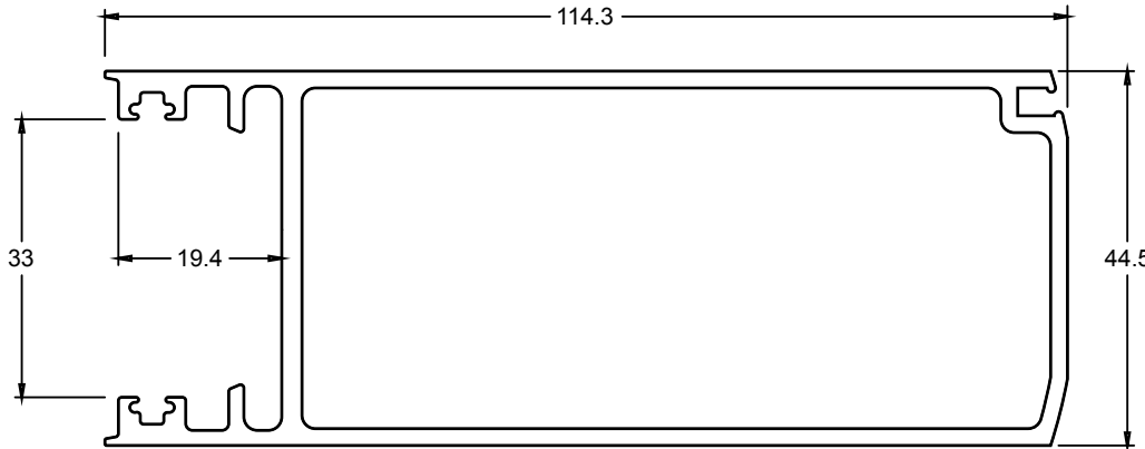
TJ436 SLIDING STILE
