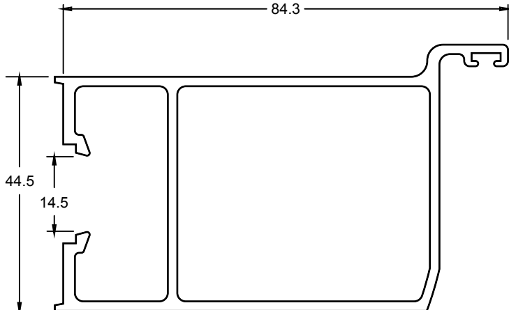
TJ444 MEETING STILE
