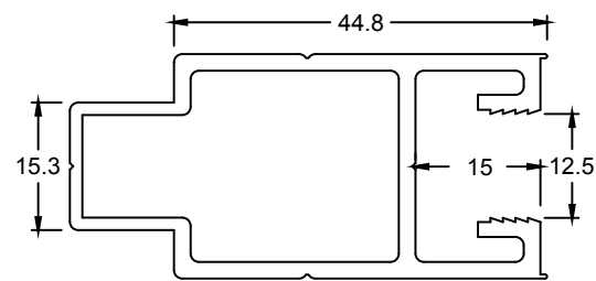
SWD057 MALE STILE
