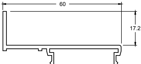
CDG6516 AWNING STOP
