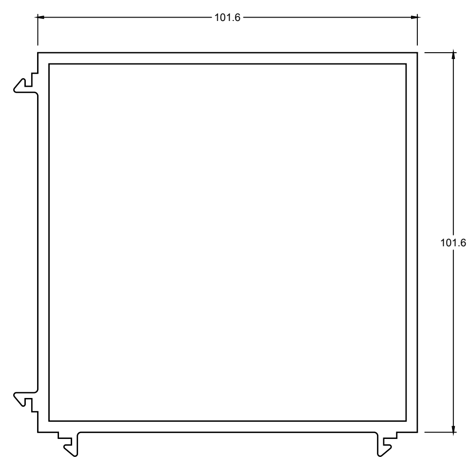
TJ319 CORNER POST
