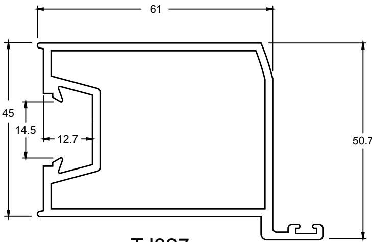
TJ327 MEETING STILE
