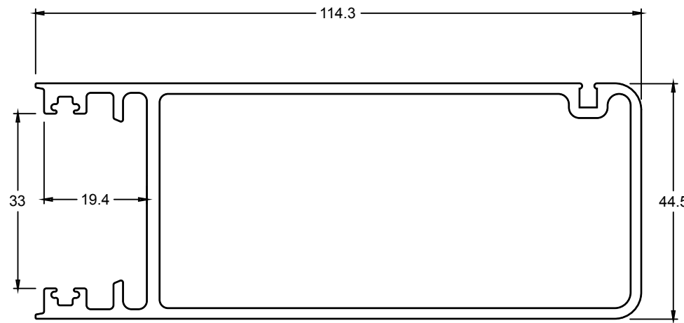
TJ428 LOCK STILE
