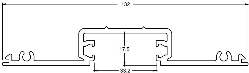
CDG6504 GLAZING ADAPTOR
