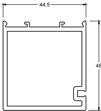
TJ204 SLIDING STILE
