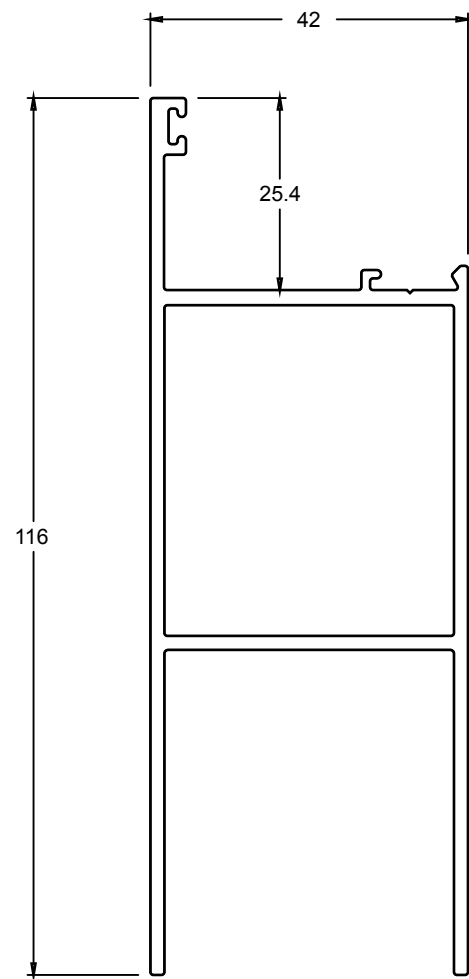
TJ420 BOTTOM RAIL
