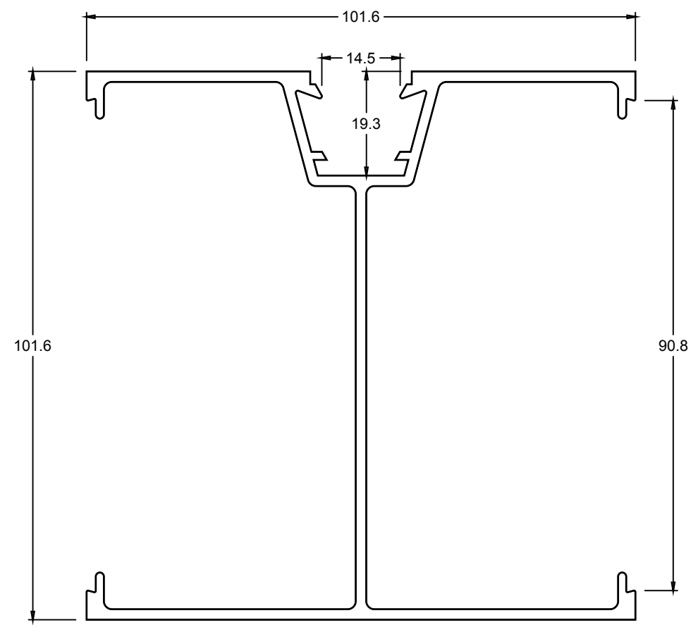
TJ308 CORNER POST
