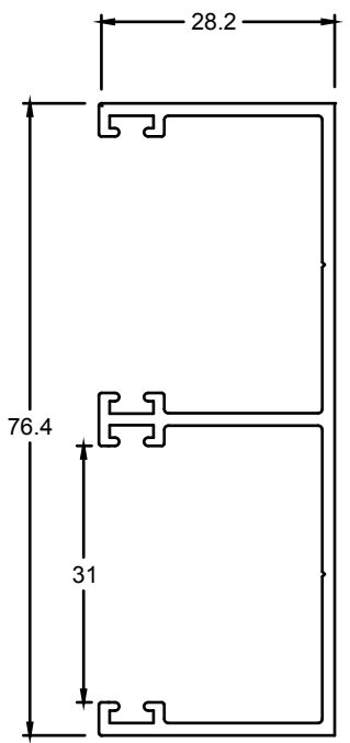
DH117 DOUBLE GLAZED PLANT ON JAMB
