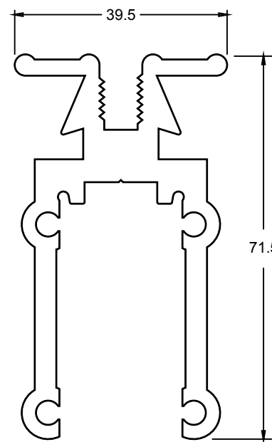
1817 OPEN POCKET SPIGOT
