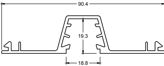
TJ304 GLAZING ADAPTOR
