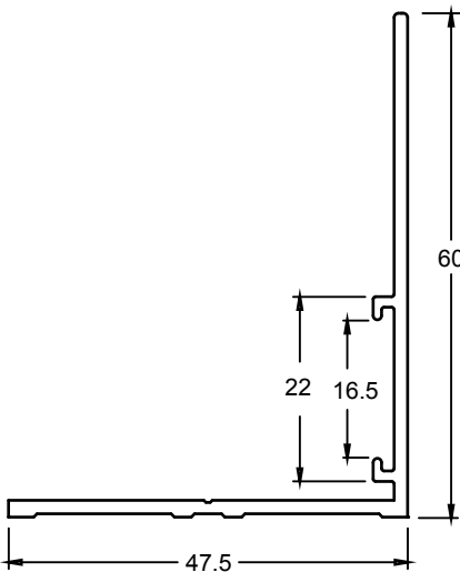
LVB060 60mm WEATHER BAR
