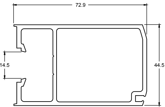
TJ440 LOCK STILE
