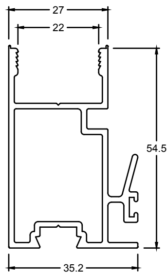
DH253 INTERLOCK TOP SASH DG
