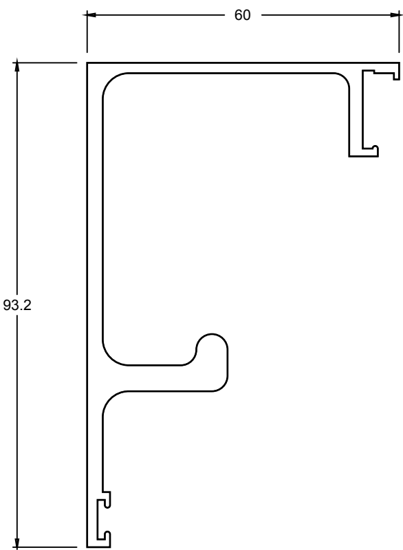
TJ323 DOOR TRACK
