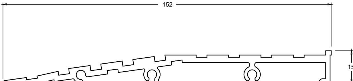
TJ339 WHEELCHAIR THRESHOLD
