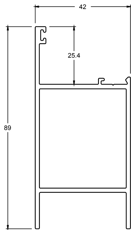
TJ419 TOP RAIL
