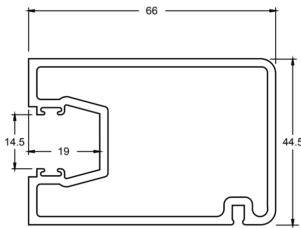
HV322 SLIDING STILE
