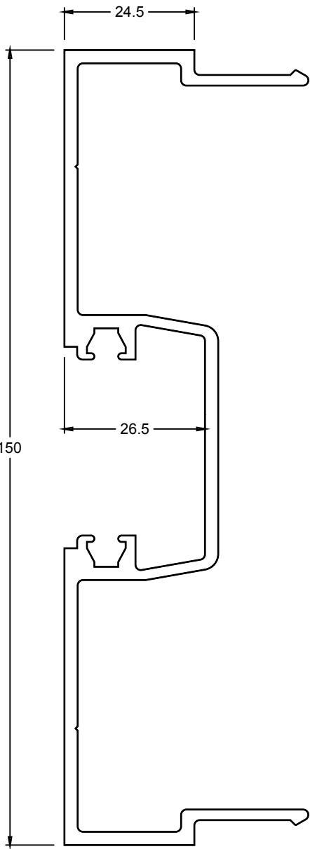
CDG6510 SPLIT MULLION MALE
