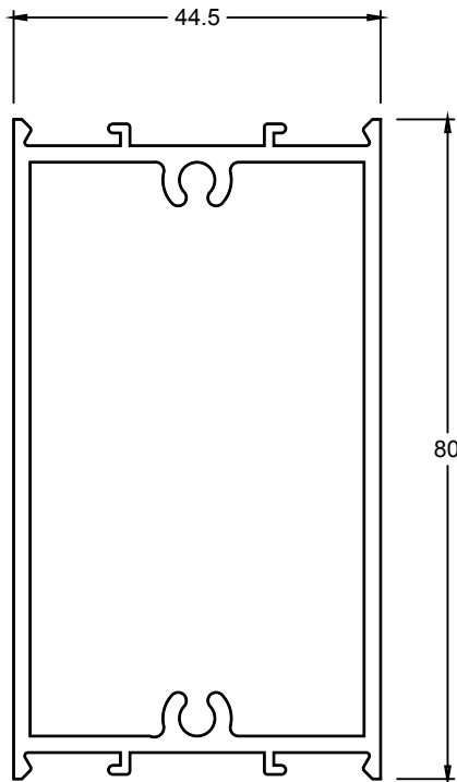
TJ209 MID RAIL
