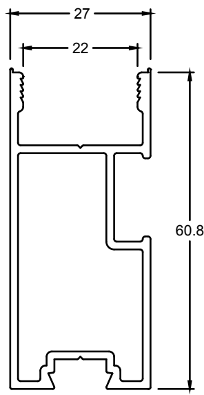
DH258 RAIL DG
