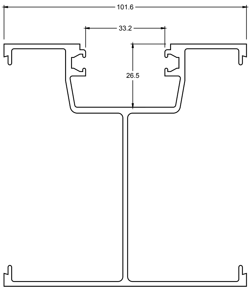
CDG4305 DOUBLE GLAZED CORNER POST
