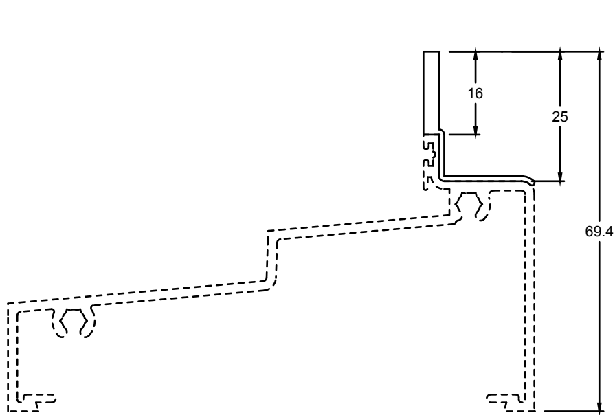
DH115 H/PERFORMANCE SILL ADAPTOR
