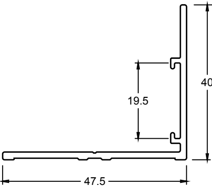
LVB040 40mm WEATHER BAR
