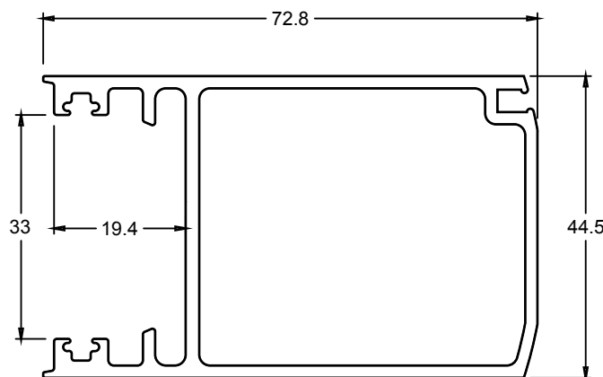
TJ418 SLIDING STILE
