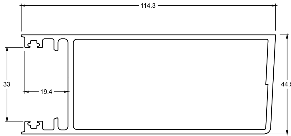
TJ435 HINGE STILE
