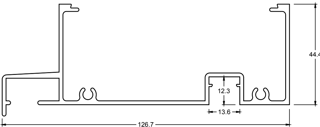
LCV002 LOUVRE FRAME HEAD
