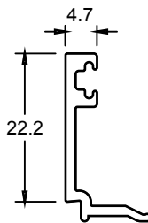
TJ227 DOUBLE GLAZED BEAD
